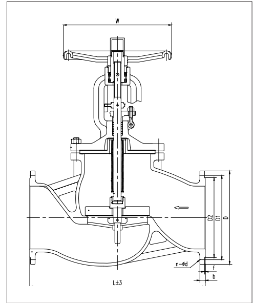
DN200-400
